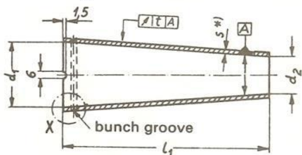
Type B1 without bull-nose
