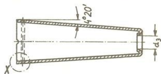
Type B2 with bull-nose
